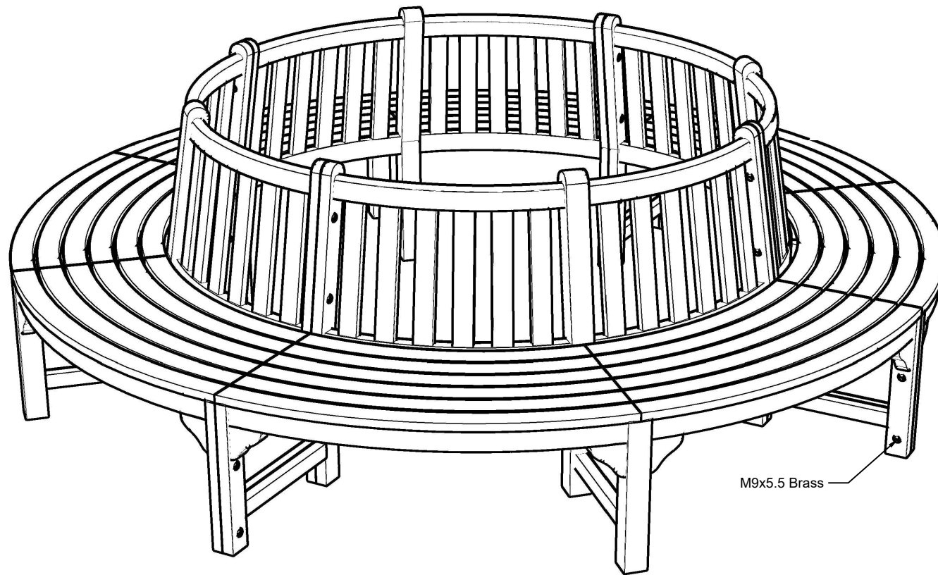
ISOMETRIC
